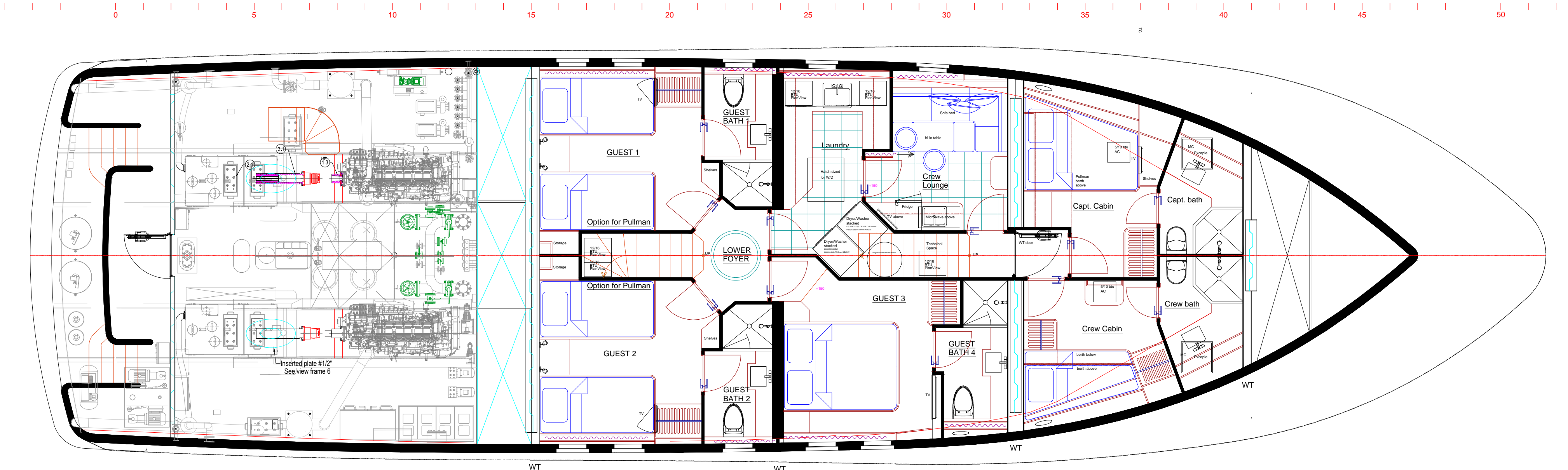
STANDARD LOWER DECK LAYOUT WITH OPTIONAL AND OWNER SUPPLIED ITEMS
