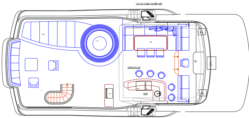
STANDARD LAYOUT WITH OPTIONAL AND OWNER SUPPLIED ITEMS
