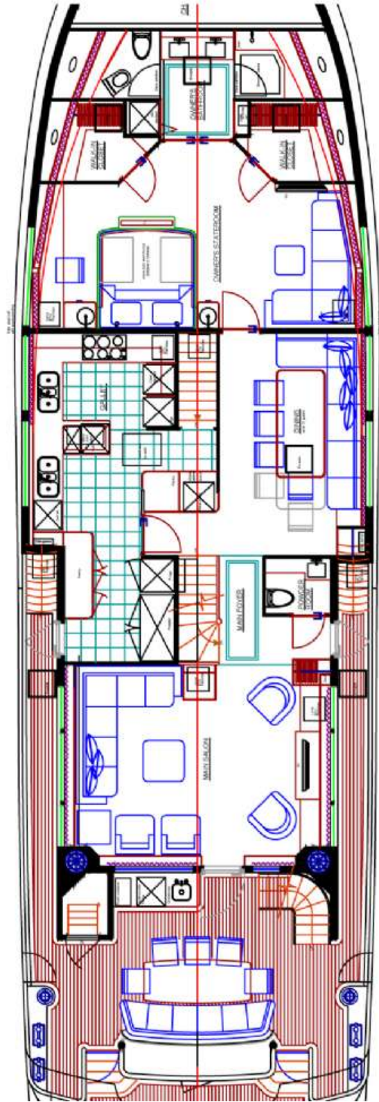
STANDARD LAYOUT "MONACO" WITH OPTIONAL AND OWNER SUPPLIED ITEMS
