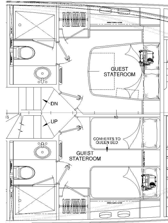
Starboard Twin berth Stateroom 2
