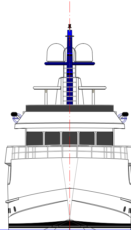
BOW VIEW
