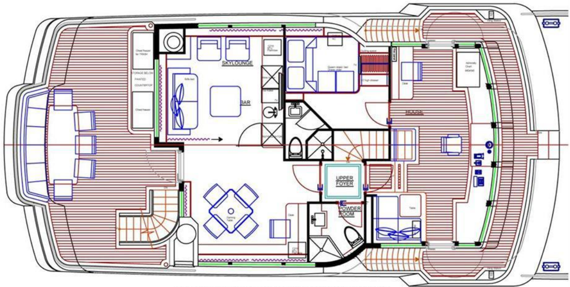
CAPTAIN'S CABIN UP OPTION
