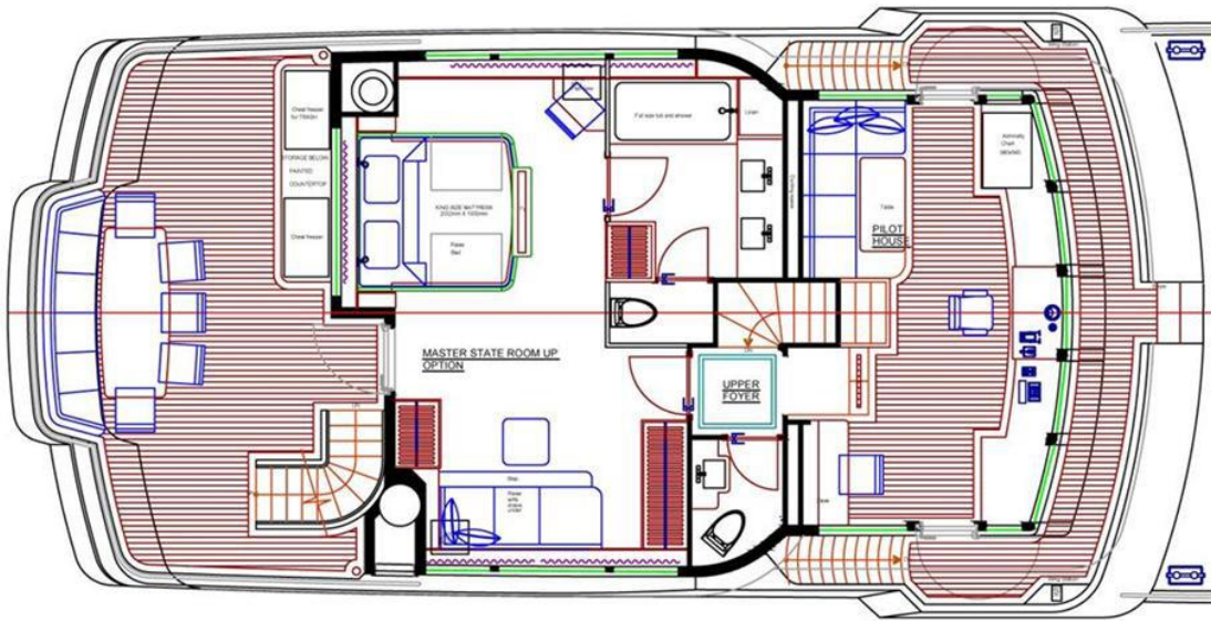
Owner Behind Wheelhouse Layout Tub / Shower
