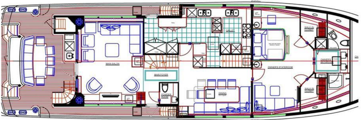
STANDARD LAYOUT "MONACO" WITH OPTIONAL AND OWNER SUPPLIED ITEMS
