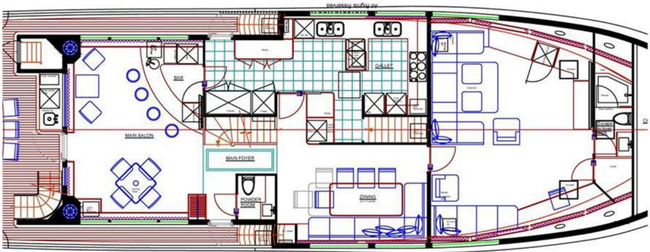
Owner Up / Forward TV Lounge & Office / Aft Bar / Gaming Room
