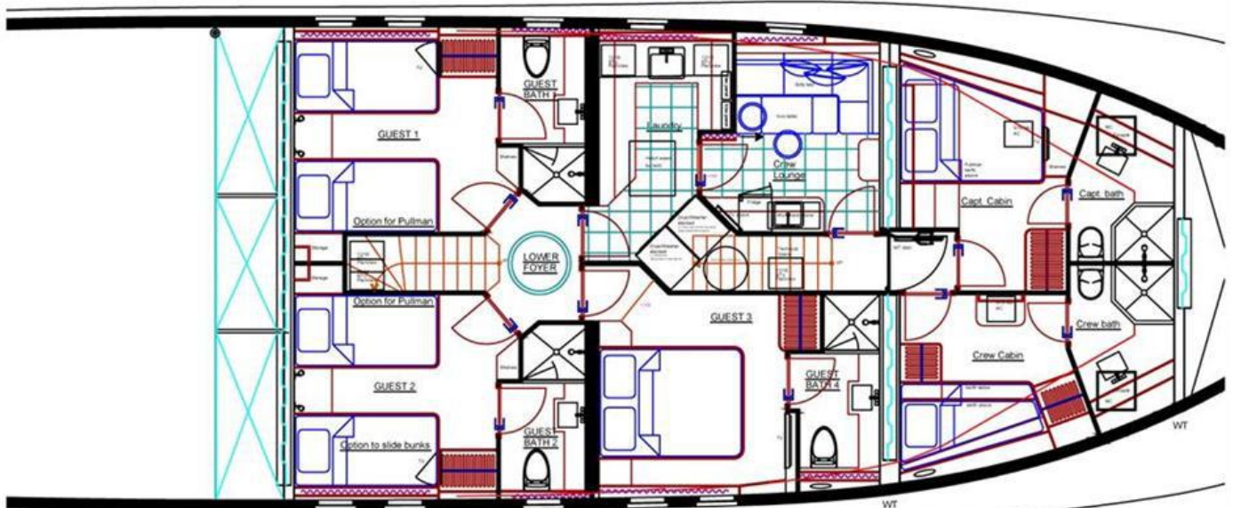
STANDARD LOWER DECK LAYOUT WITH OPTIONAL AND OWNER SUPPLIED ITEMS
