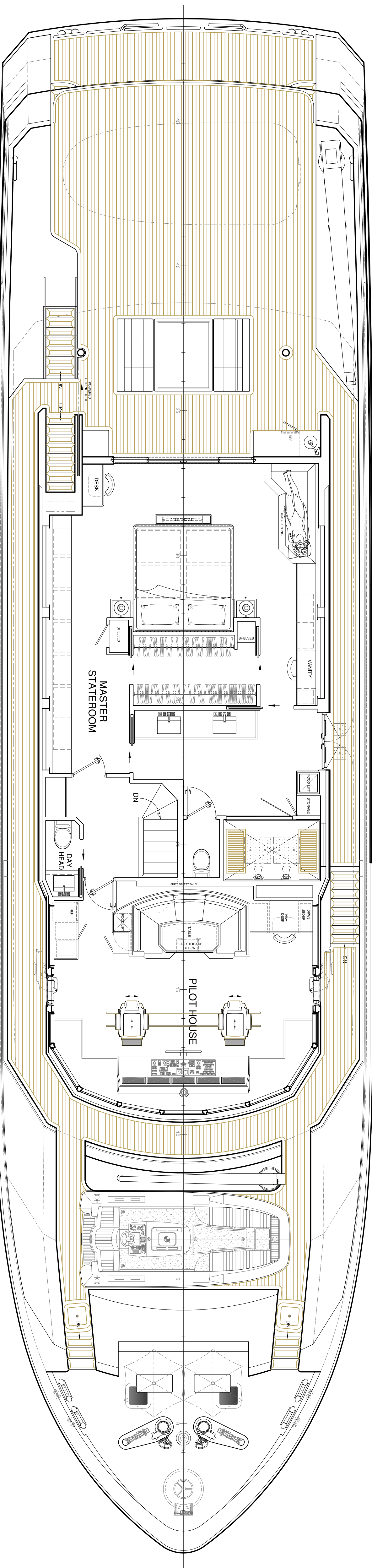
BRIDGE DECK ORIGINAL
